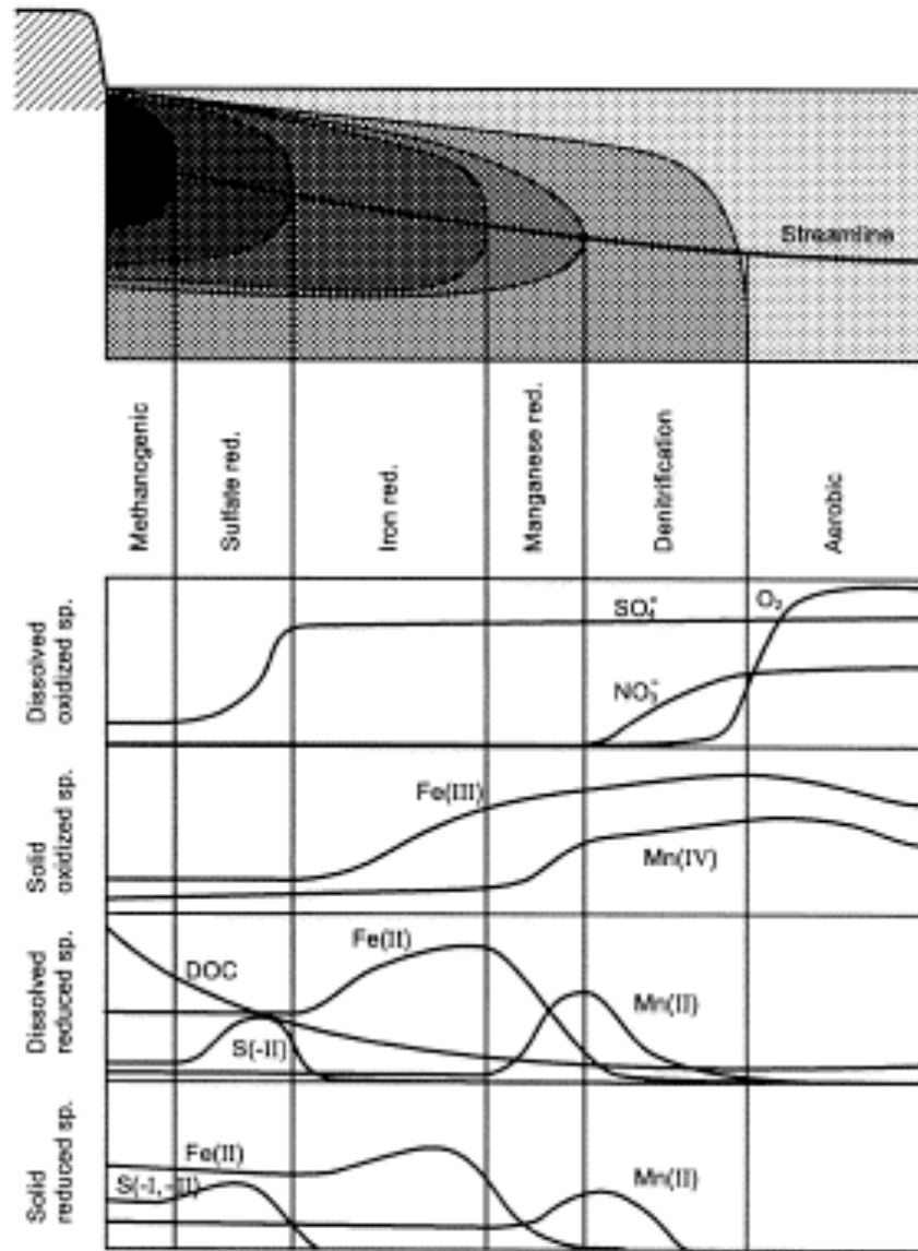
Figure S2. Schematic redox zonation in an originally aerobic aquifer downgradient from a landfill, and the distribution of redox-sensitive species along a streamline in the plume. The value axes are not to scale. Source: Christensen, T. H., et al. Appl. Geochem. 2001 , 16 , 659–718. Used with permission from Elsevier.
